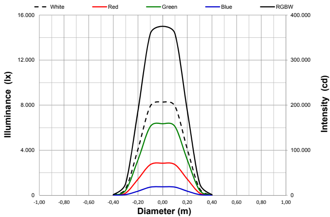
A.leda B-EYE K10 CC Illuminance Distribution Minimum Zoom - distance = 5m
