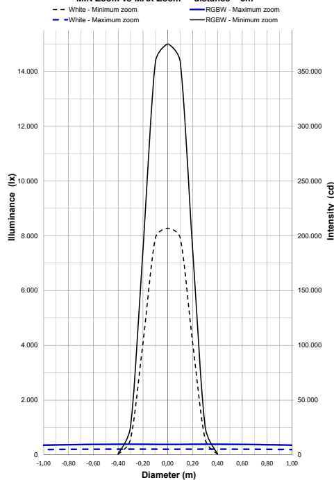
A.leda B-EYE K10 CC Illuminance Distribution MIN Zoom vs MAX Zoom - distance = 5m
