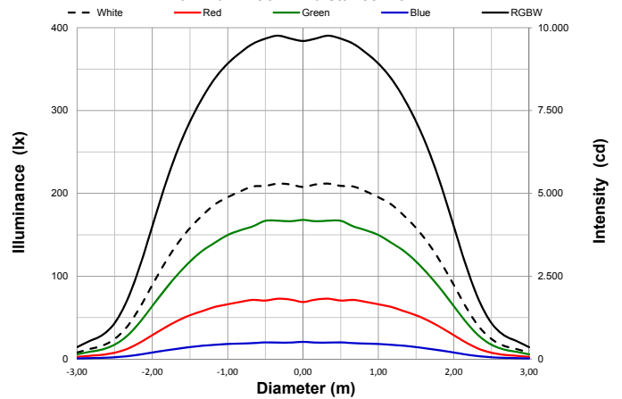
A.leda B-EYE K10 CC Illuminance Distribution Maximum Zoom - distance = 5m
